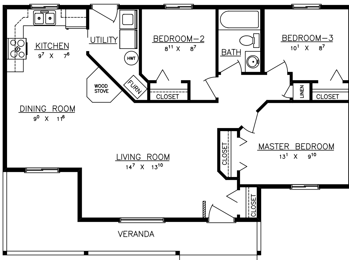
FLOOR PLAN
